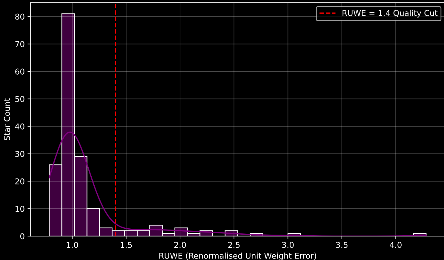
GAPOGEE DR17 Field [181+42_MGA] RUWE Distribution (n= 171)
