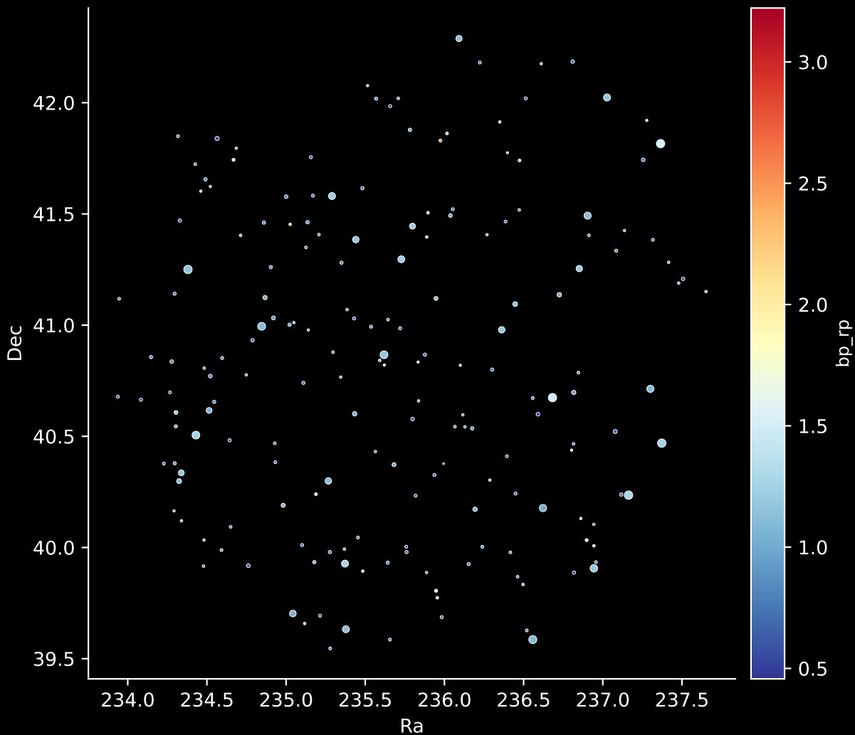
APOGEE DR17 Field: [181+42_MGA] Stars: 184
