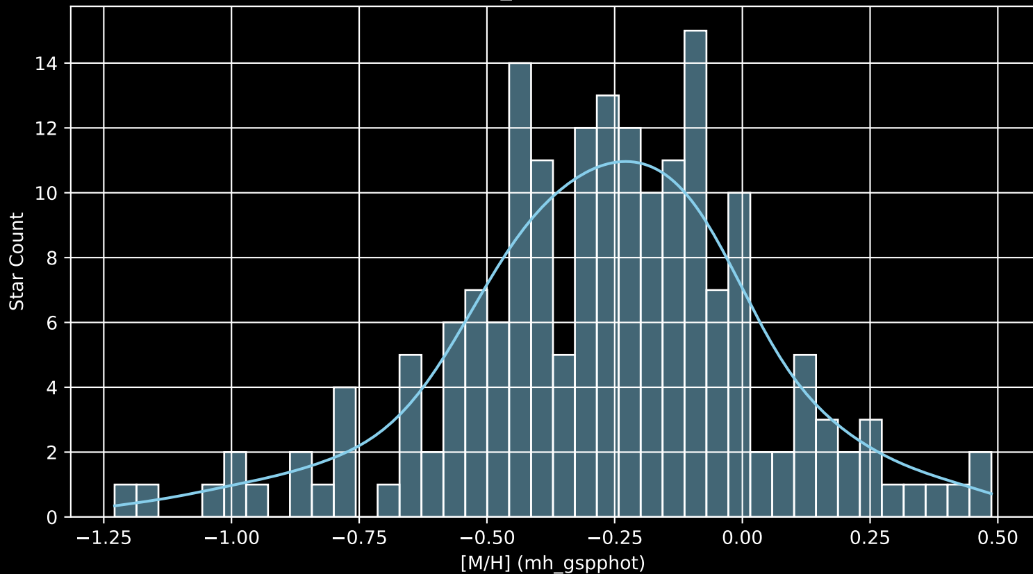
APOGEE DR17 Field: [181+42_MGA [M/H] (mh_gspphot) (n= 183)
