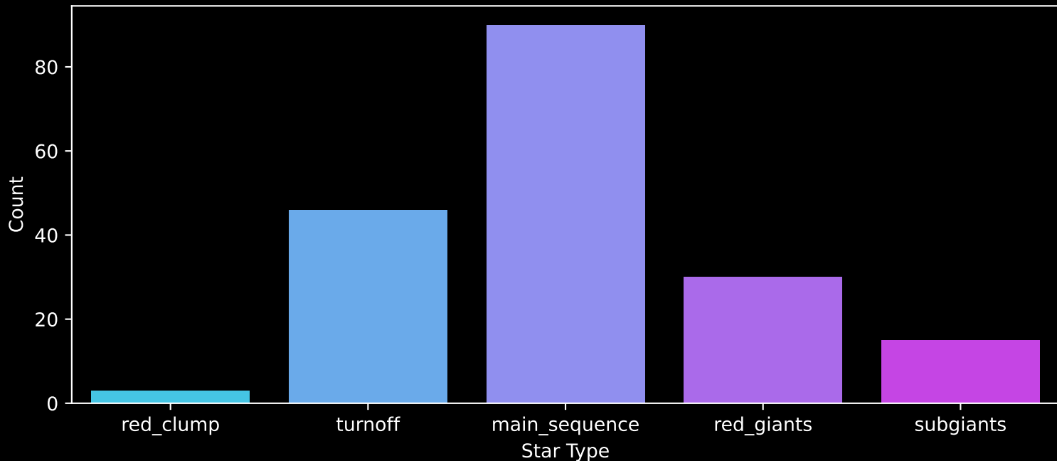
APOGEE DR17 Field: [181+42_MGA] Count plot of Star Type
