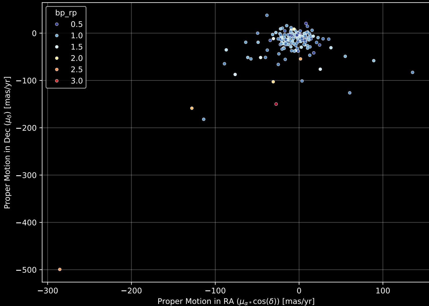
APOGEE DR17 Field: [181+42_MGA] Proper Motion Diagram (n= 184)
