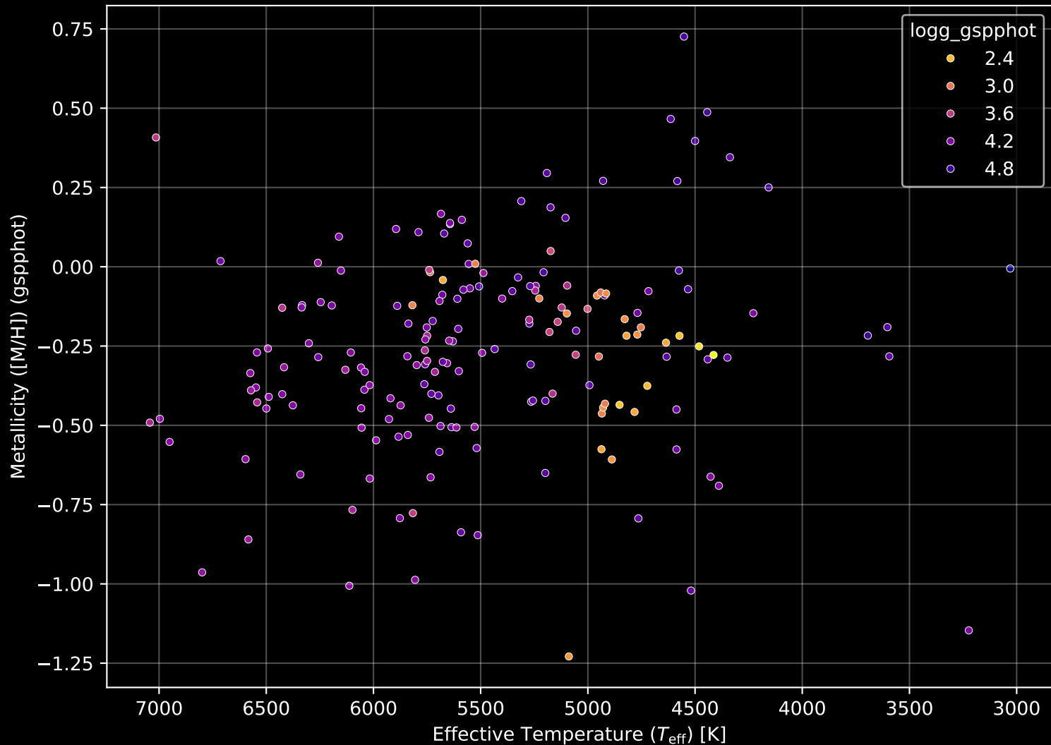
APOGEE DR17 Field: [181+42_MGA] Stellar Population Parameters (n= 184)
