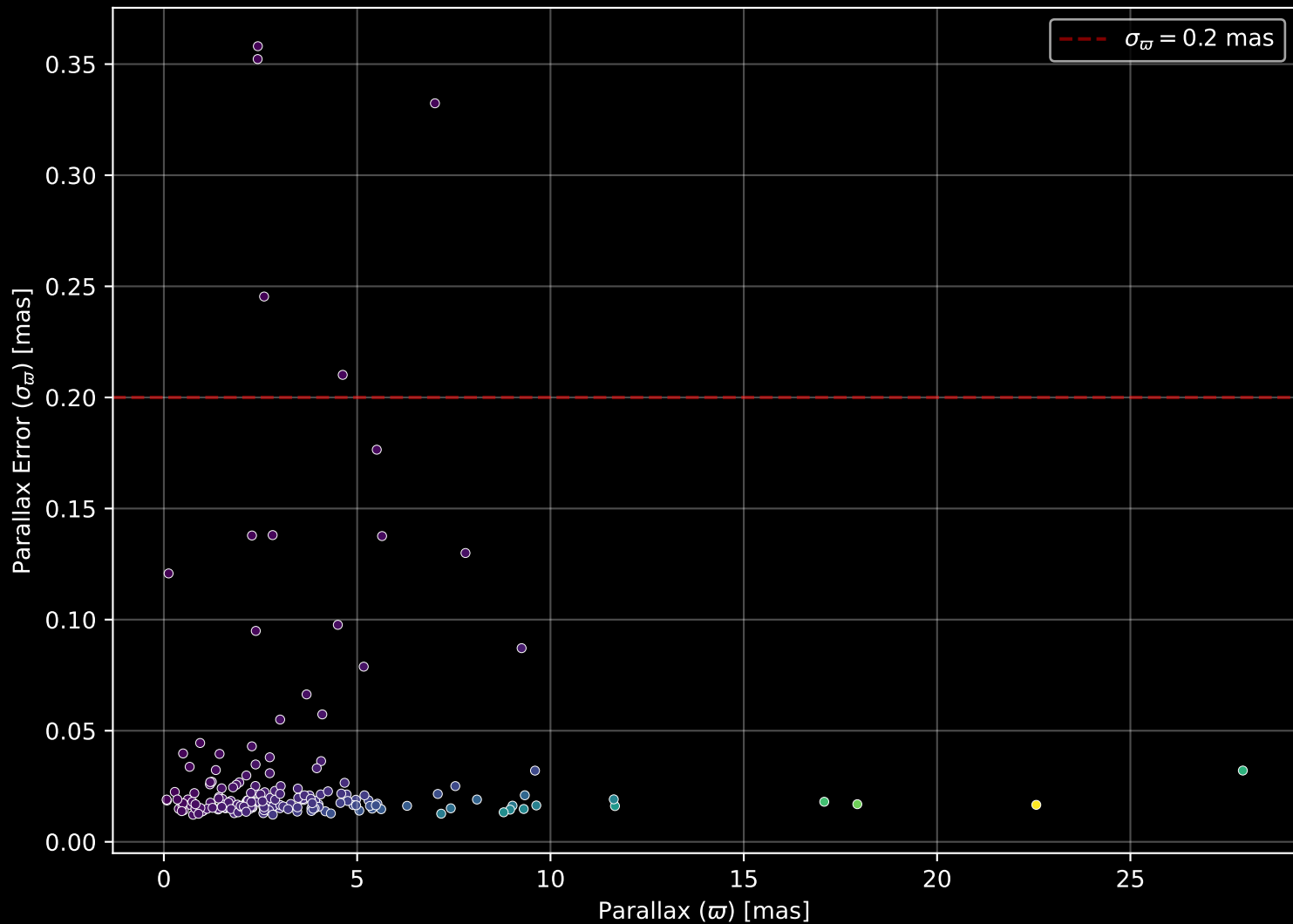
APOGEE DR17 Field: [181+42_MGA] Parallax Quality (n= 184)
